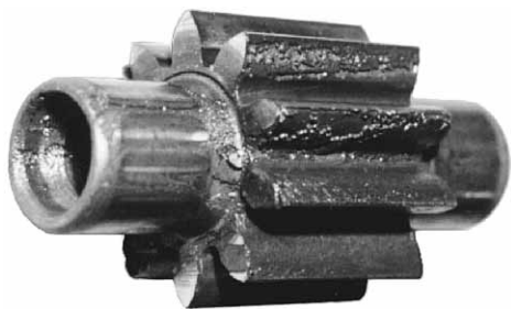
This gear was damaged by orange juice that got into the hydraulic system.
