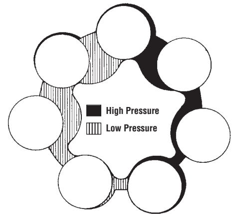
Gerotor Design
