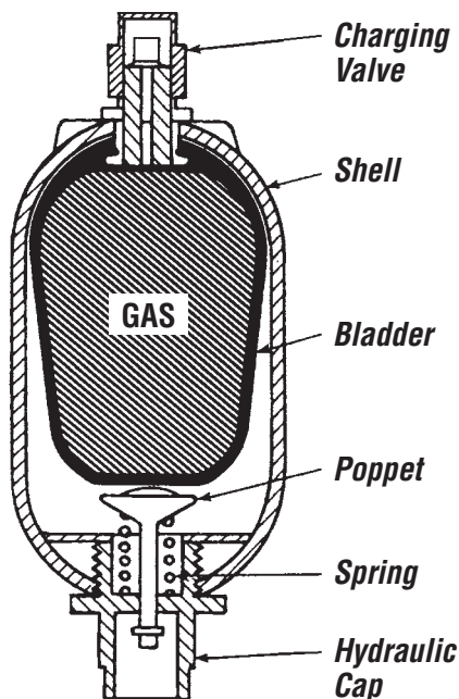
The Bladder Accumulator
