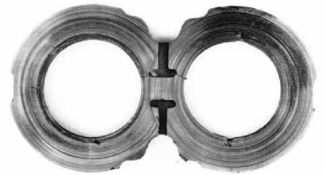
Phonographing on wearplate
