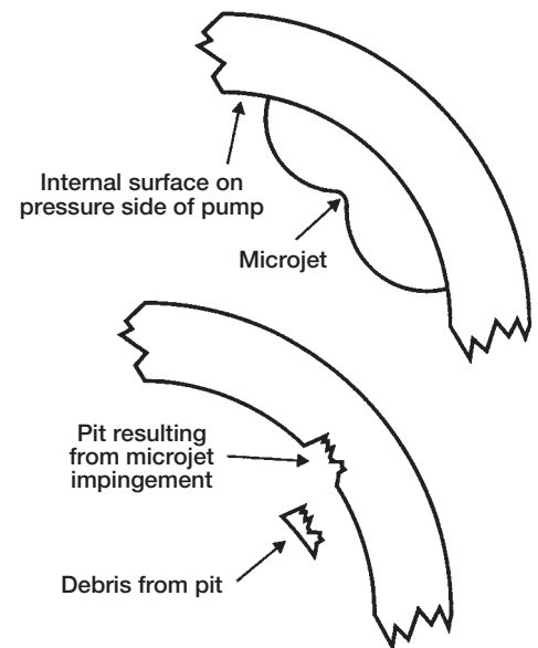
Pitting results from the collapse of air or gas bubbles on the internal surface of the pump.
