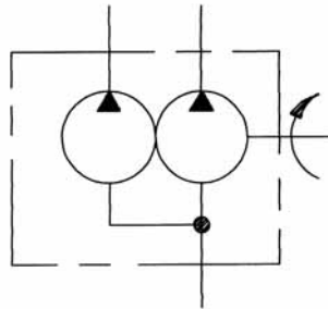
Tandem pump uni-rotational fixed displacement
