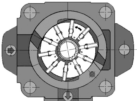
Cross section of vane pump
