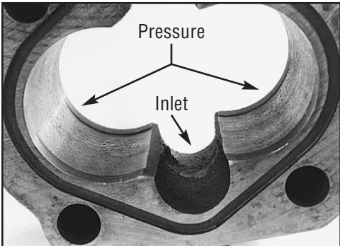
This pump housing shows a deep gear path (.014") caused by overpressurization. Acceptable cutout must measure .005" or less to provide satisfactory service. High pressure forces the pump gears to the inlet or low pressure side of pump. When excessive pressure occurs, the gears deflect causing abnormal gear cutout.
