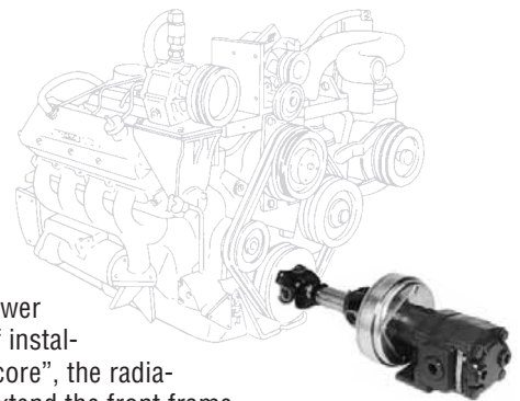
Crankshaft driven clutch pump.
