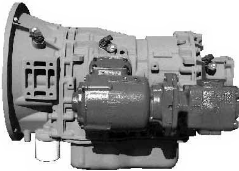
Muncie CS Series PTO and PK Series gear pump mounted to an Allison® automatic transmission.
