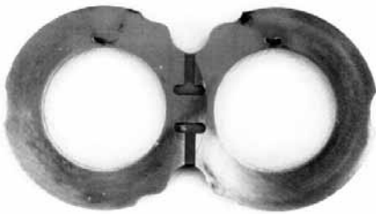
Wearplate showing pitting from cavitation
