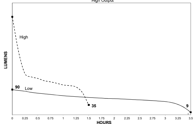
PERFORMANCE CURVE High Output
